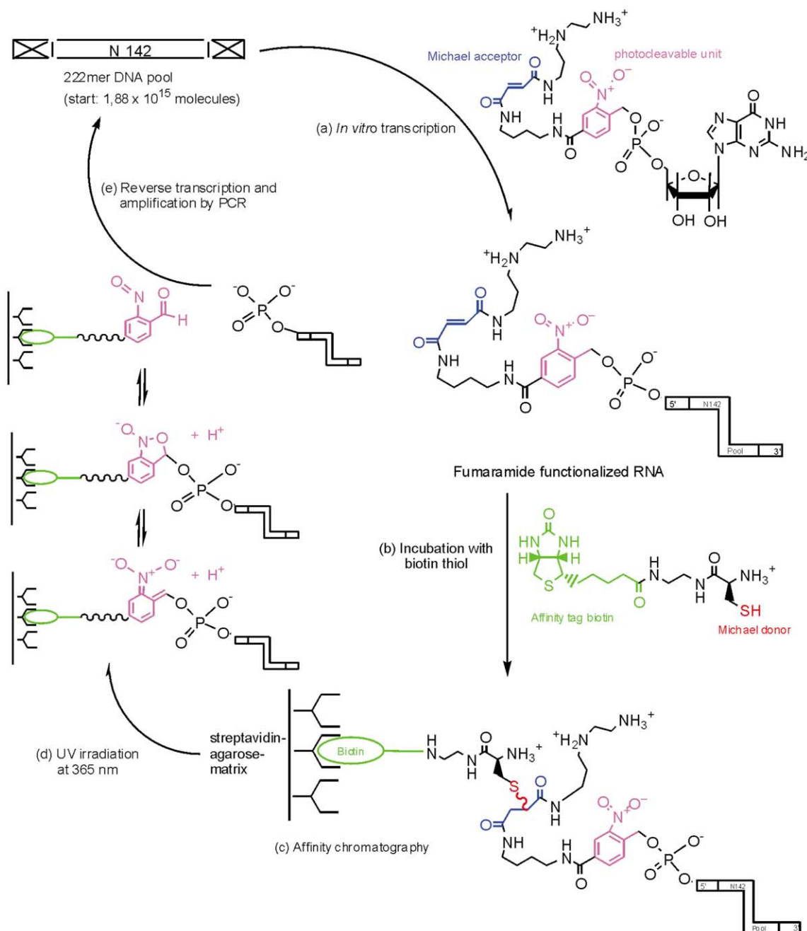
Scheme 1. In vitro selection of catalytic RNA for the Michael reaction: (a) in vitro transcription of randomized DNA template with fumaramide-derivatized guanosine generates fumaramide-functionalized RNA libraries; (b) Michael reaction of biotinylated cysteine thiol with the RNA library leads to biotinylation of active RNAs; (c) inactive RNAs are removed by affinity chromatography on streptavidin agarose; (d) active RNAs are isolated after photocleavage; (e) reverse transcription of the active RNAs followed by PCR amplification of the cDNA library affords DNA pool for the next cycle.
