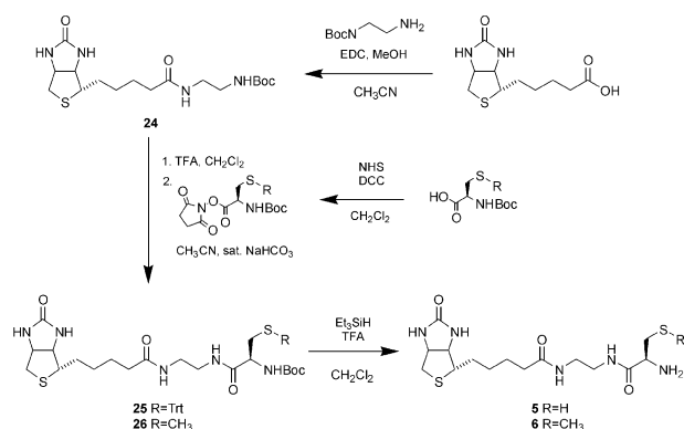
Scheme 5. Synthesis of biotin cysteine thiol 5 and S-methylated analog 6 .
