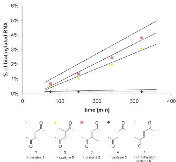
Figure 3. Time course of the background reaction of the Michael reaction between fumaramide derivatized RNA-library (pool-RNA derivatized with 1–3) and biotinylated cysteine 5. The reactions were carried out under selection conditions [50 mM K-MOPS (pH 7.4), 200 mM NaCl, 5 mM MgCl 2 , room temperature] at concentrations of [modified RNA] = 1 \mu M and [biotinylated cysteine] = 30–50 mM. As negative controls, the same experiment was performed using succinamide 4 derivatized pool-RNA or using S -methylated cysteine 6.
