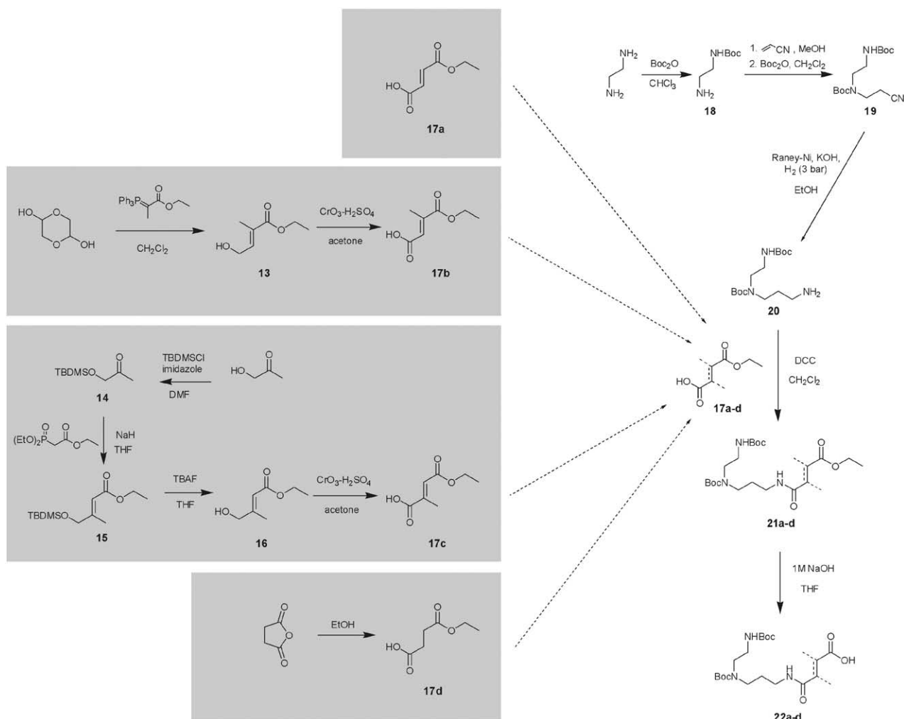
Scheme 3. Synthesis of the fumaramide and succinamic acid derivatives 22a–d .
