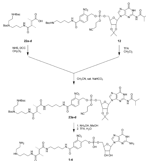
Scheme 4. Synthesis of fumaramide-derivatized guanosines 1–4 .
