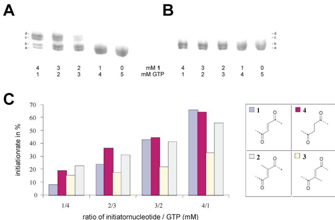
Figure 2. Enzymatic incorporation of initiator nucleotides 1–4 . (A) Representative autoradiogram of a transcription reaction of a synthetic 114 bp DNA-template in the presence of initiator nucleotide 1 run by T7-RNA-polymerase. Bands a, b, c, d represent the desired transcripts. Band a: unmodified RNA 92-mer ( n -mer) transcript, band b: unmodified RNA 93-mer transcript ( n + 1-mer), the additional nucleotide could be A, C, G or U), band c: fumaramide-RNA conjugate ( n -mer), band d: fumaramide-RNA conjugate ( n + 1-mer). (B) Gelelectrophoretic separation and autoradiography of the same transcripts as in A after exposure to UV light at 365 nm for 3 h. (C) Rate of incorporation for initiator nucleotides 1–4 .
