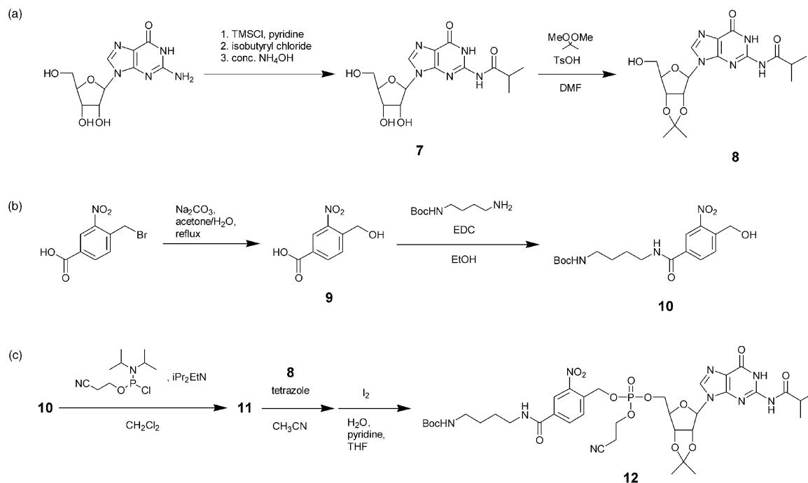
Scheme 2. (A) Synthesis of protected guanosine 8 ; (B) synthesis of the photocleavable unit 10 ; (C) coupling of guanosine and photocleavable unit to give derivatized guanosine 12 .
